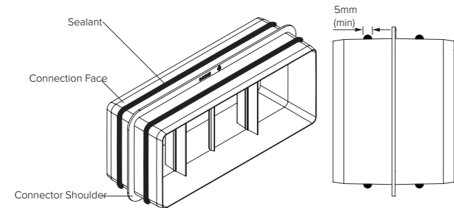
FIGURE 12: FITTING PVC BAND
